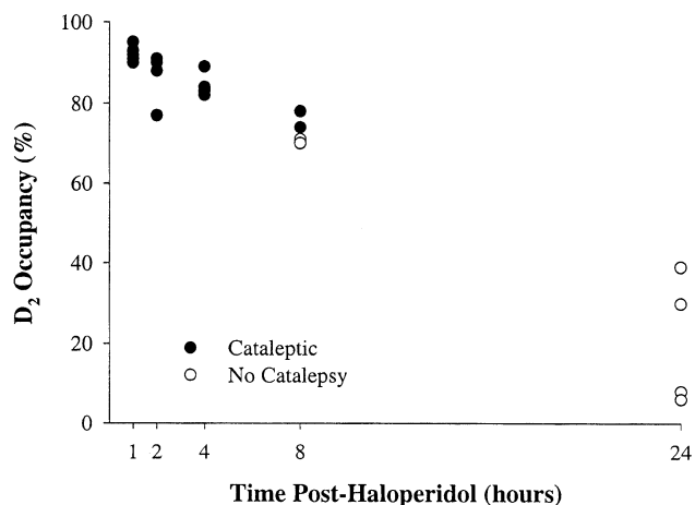
Figure 2. Time effect relationship between percent D 2 receptor occupancy and catalepsy following a single dose of haloperidol in rats. Haloperidol (0.5 mg/kg, s.c.) was administered. Non-cataleptic animals are presented as open circles and cataleptic animals as filled circles. Each circle represents one animal (total n = 25). Catalepsy scores, expressed as median \pm semi-interquartile range, were 5.0 \pm 0.5 (1 hr), 5.0 \pm 0.0 (2 hrs), 5.0 \pm 0.0 (4 hrs), 3.0 \pm 1.5 (8 hrs), and 0.0 \pm 1.5 (24 hrs), respectively. There was a statistically significant ( r = .83 ; p < .05 ) positive correlation between catalepsy and percent D 2 receptor occupancy.
